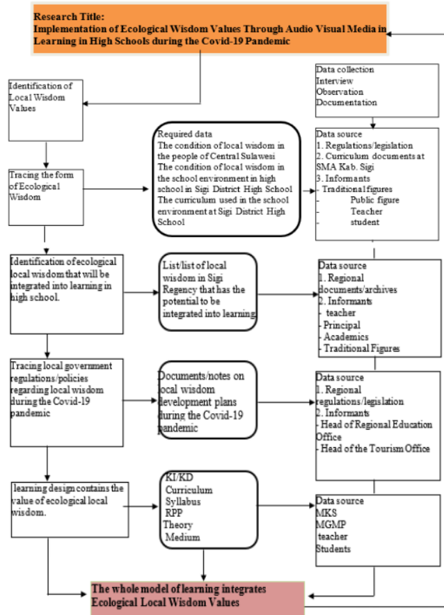
Figure 1. Research Flowchart
